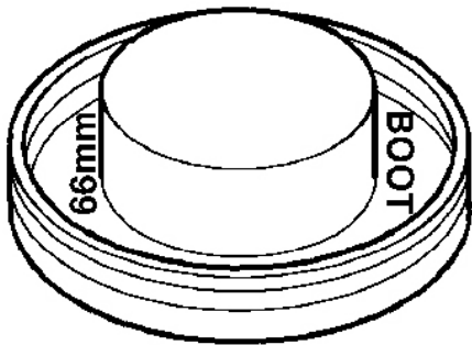
Figure 46. 2x66mm Piston and Piston Boot Insertion Tool
