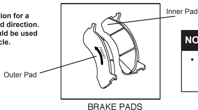
Figure 10. HX-7A1-EE Brake Pads
