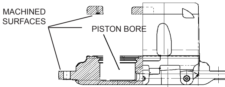
Figure 4. Caliper Housing
