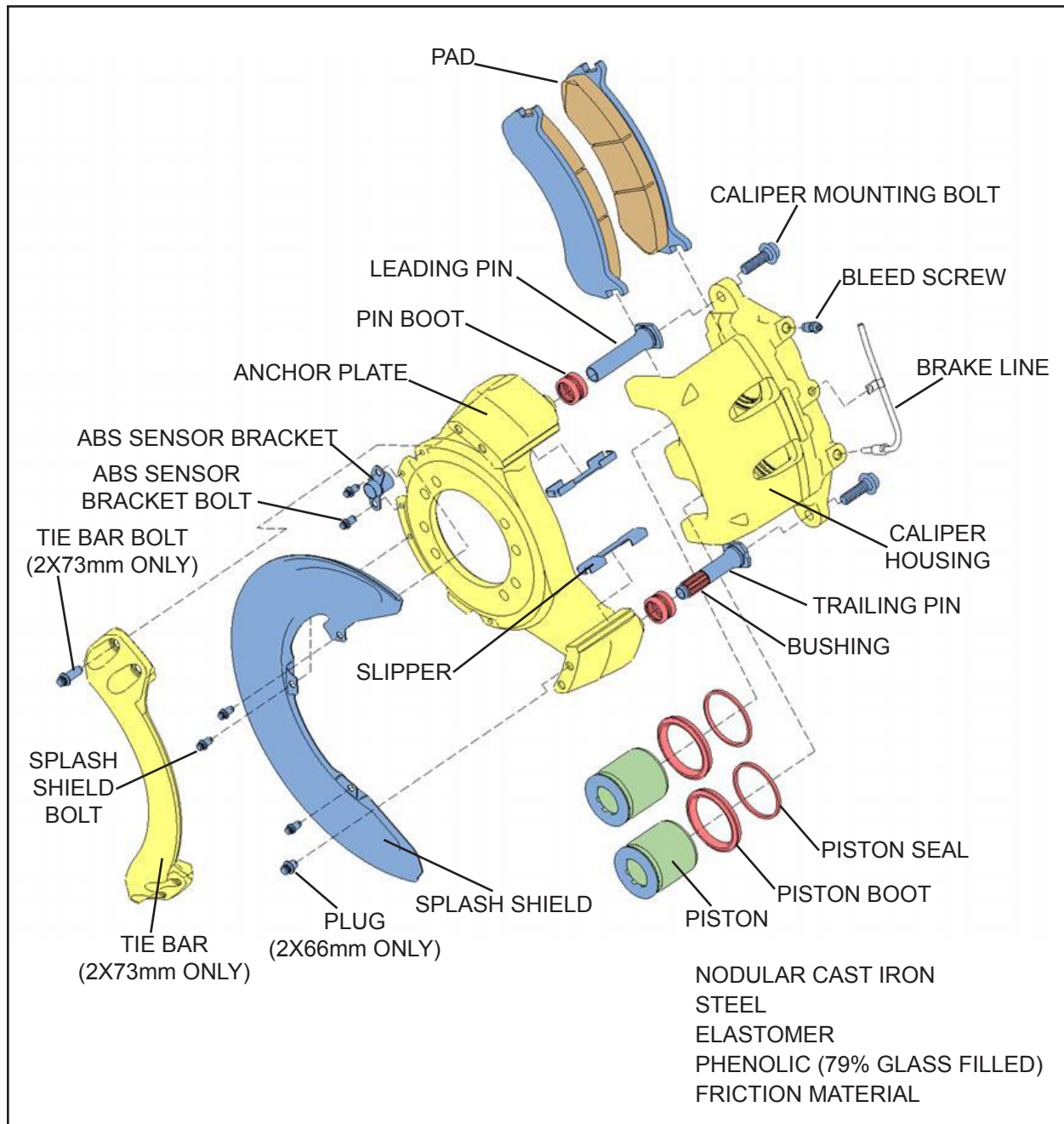
Figure 1. Pin Slide Disc Brake Components
