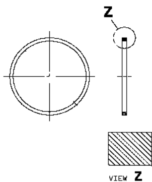
Figure 6. Piston Seal
