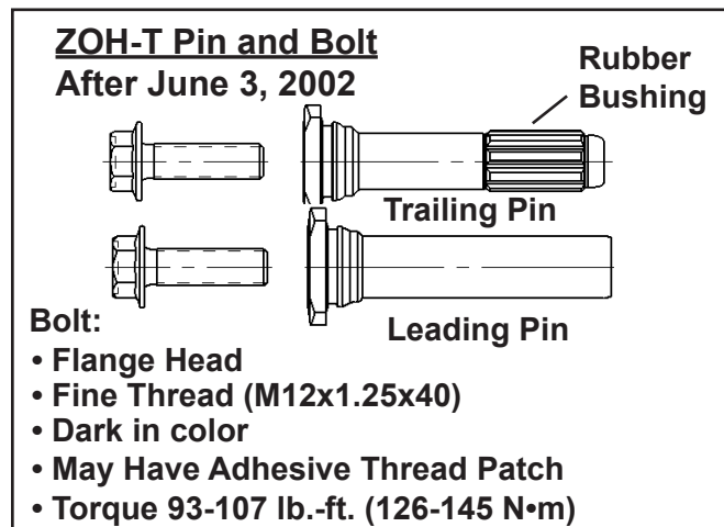
Figure 12. ZOH-T Caliper Mounting Bolt and Pins
