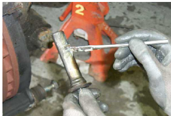
Figure 36. Lubricate Leading and Trailing Pins
