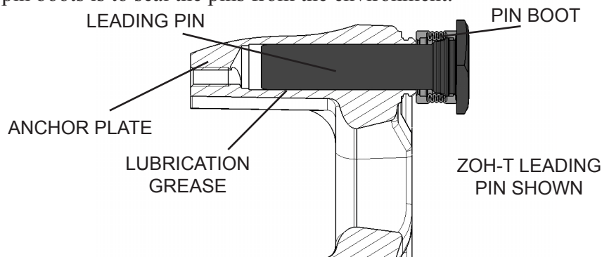
Figure 14. ZOH-T Leading Pin and Pin Boot Shown Installed In Anchor Plate
