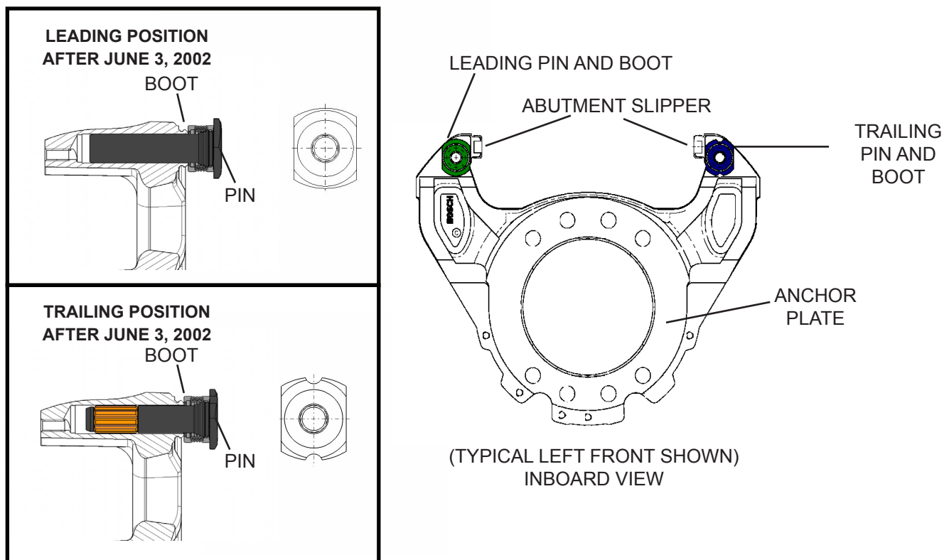
Figure 13. Typical Anchor Plate Assembly
