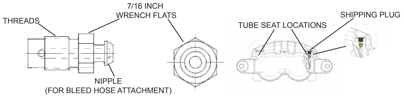
Figure 8. Bleed Screw and Tube Seat
