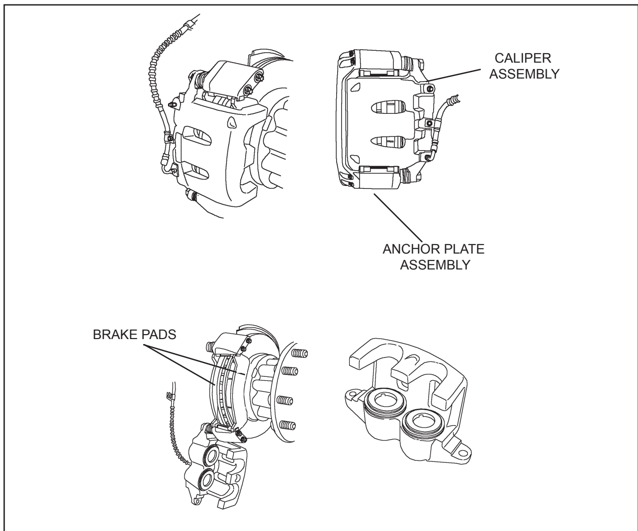
Figure 2. Pin Slide Disc Brake Components
