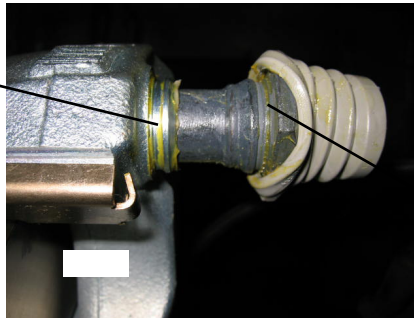
Figure 42. Installing Pin Boot over Pin Flange
