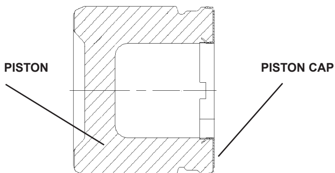
Figure 5. Piston Assembly
