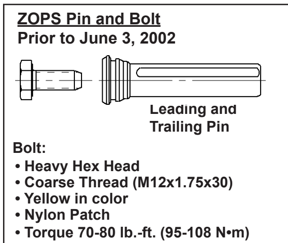
Figure 11. ZOPS Caliper Mounting Bolt and Pins
