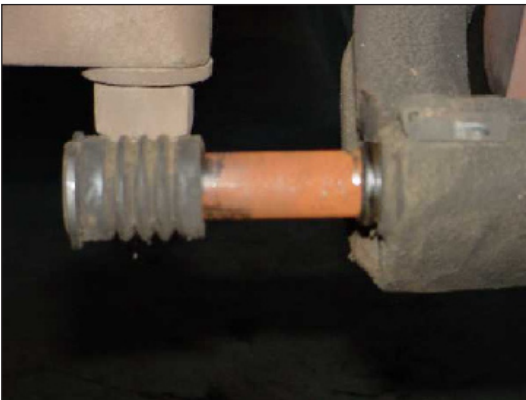
Figure 31. Example of Anchor Plate Pin with Heavy Corrosion
