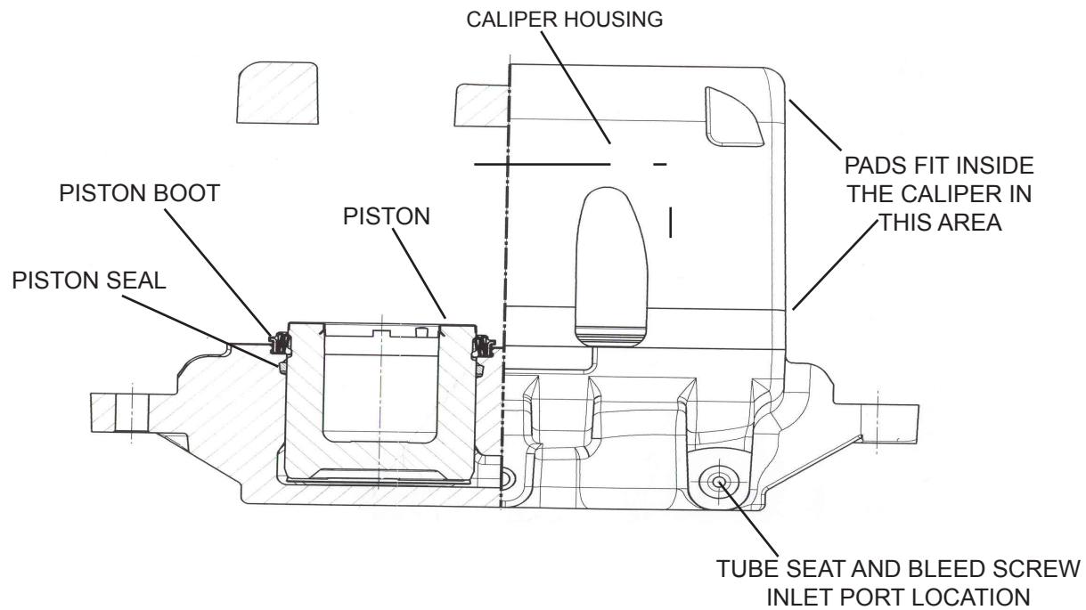
Figure 3. Caliper Assembly
