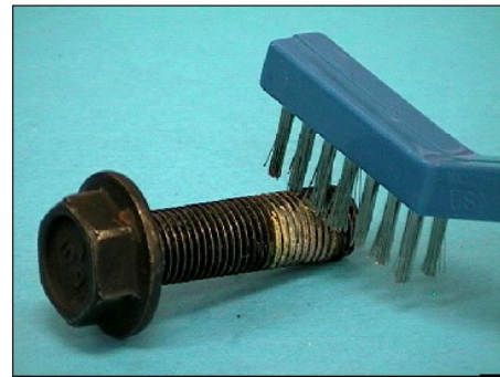
Figure 26. Use a Steel Brush to Buff Away the Existing Adhesive Residue
